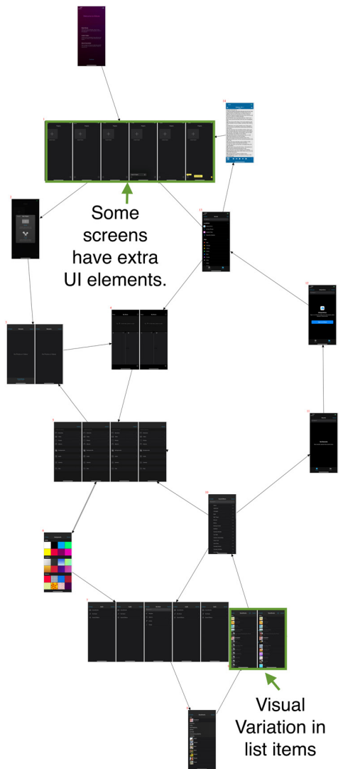
Fig. 13. Similarity transformer storyboard example—in this case, the model is able to group screens with extra UI elements and significant visual variation.
