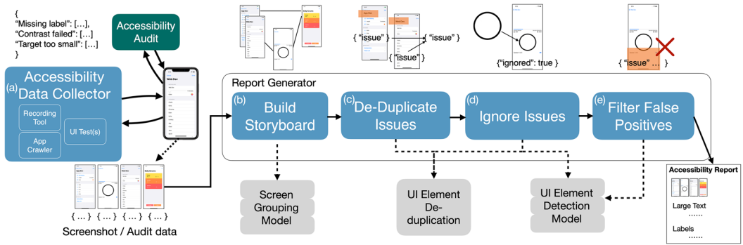
Fig. 2. Our system for accessibility report generation. A data collector (a) captures screenshots and accessibility audits, followed by a four-stage process that produces a summarized accessibility report. The stages consist of 2) “build storyboard” (b) which uses a pixel-based screen grouping model to build a storyboard of app screens, (c) and (d) “de-duplicate issues” and “ignore issues” which use UI element matching heuristics based on a UI element detection model to de-duplicate and filter out issues that QA users have ignored, and (e) “filter false positives” which removes any issues with no corresponding UI element on the screen as detected by the UI element detection model.
