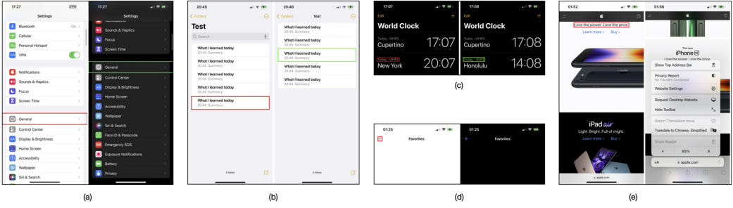
Fig. 10. Examples of correct (a) and incorrect (b–d) results from our UI element de-duplication heuristics.
