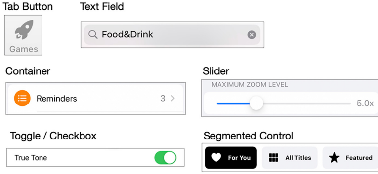
Fig. 4. UI element groupings used by UI element de-duplication heuristics to find matching UI elements in a new screen. The examples include several UI types including tab button, text field, container, toggle/checkbox, slider, and segmented control.
