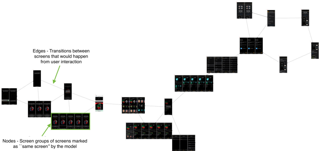
Fig. 11. Similarity transformer storyboard example. This is the full storyboard for the storyboard example in Figure 3. The nodes in this graph visualization indicate screens that were considered as “same screen” by the screen grouping model. Edges indicate transitions between screens that would happen as a result of a user interaction.
