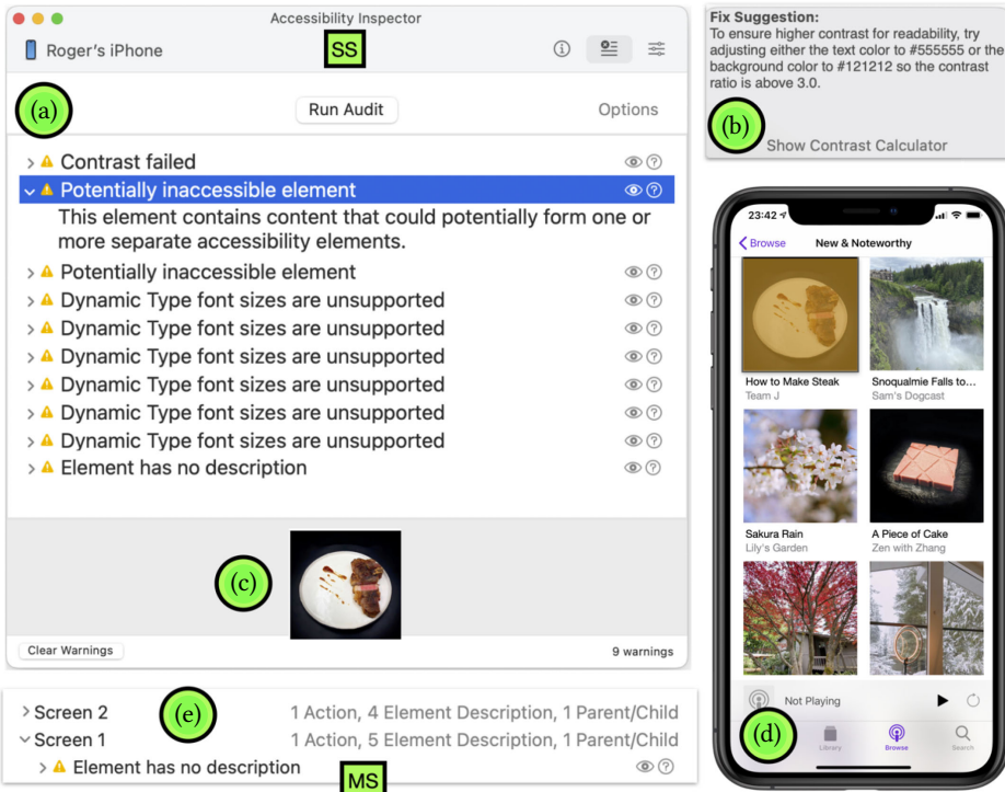
Fig. 8. Xcode's accessibility inspector [36] in single screen (SS) mode with the scanner's results for an iPhone. The Inspector has four main areas: (a) a table of detected issues for the current screen that a user requests by clicking the "run audit" button, (b) fix suggestions that appear when a user clicks on the "?" icon on a selected row, (c) a preview window with a screenshot of the impacted UI element, and (d) a device (either on a simulator or live), or an application window. Our study evaluates two modes: SS, which provides features a–d, and multi screen accessibility inspector (MS), which provides features a–e. (e) adds a history of scanned screens and headers to summarize result counts by category.
