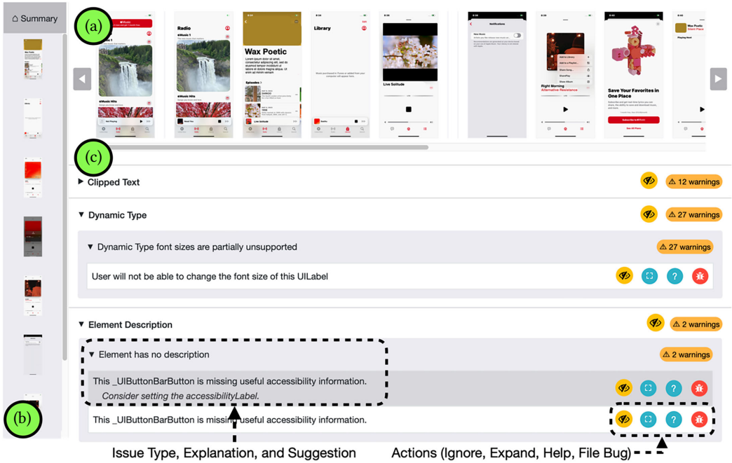
Fig. 5. The prototype interactive HTML report generated by our report generation system. The interface has three main areas: (a) a carousel displaying all screens captured in the report, (b) a menu to toggle between the “summary” view which is currently selected, and screen-by-screen views represented by thumbnail screenshots, and (c) a table of summarized results of issues found, grouped by category. The report provides actions users can take including ignoring, viewing suggestions, filing bugs, and expanding the screenshot.
